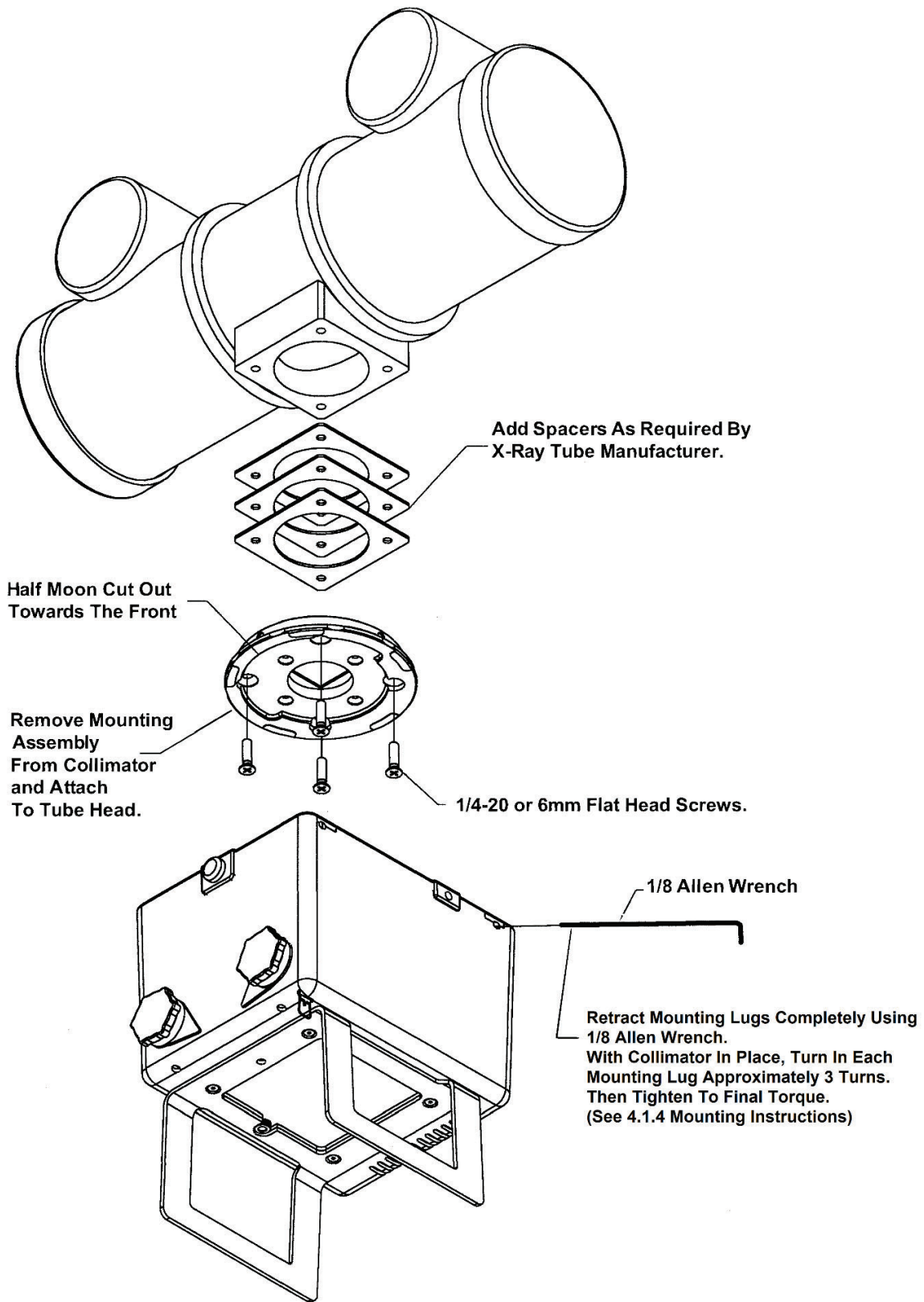
Figure 6 - CML X-Ray Tube Mounting Assembly
