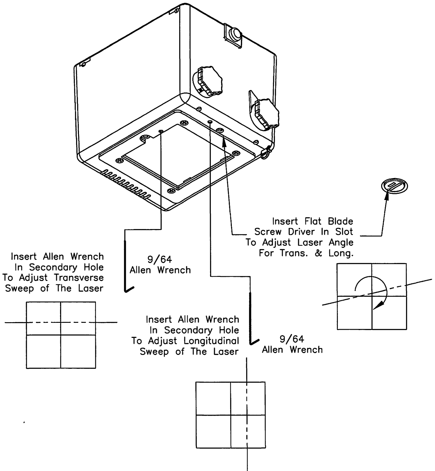
Figure 10 - Laser Adjustment
